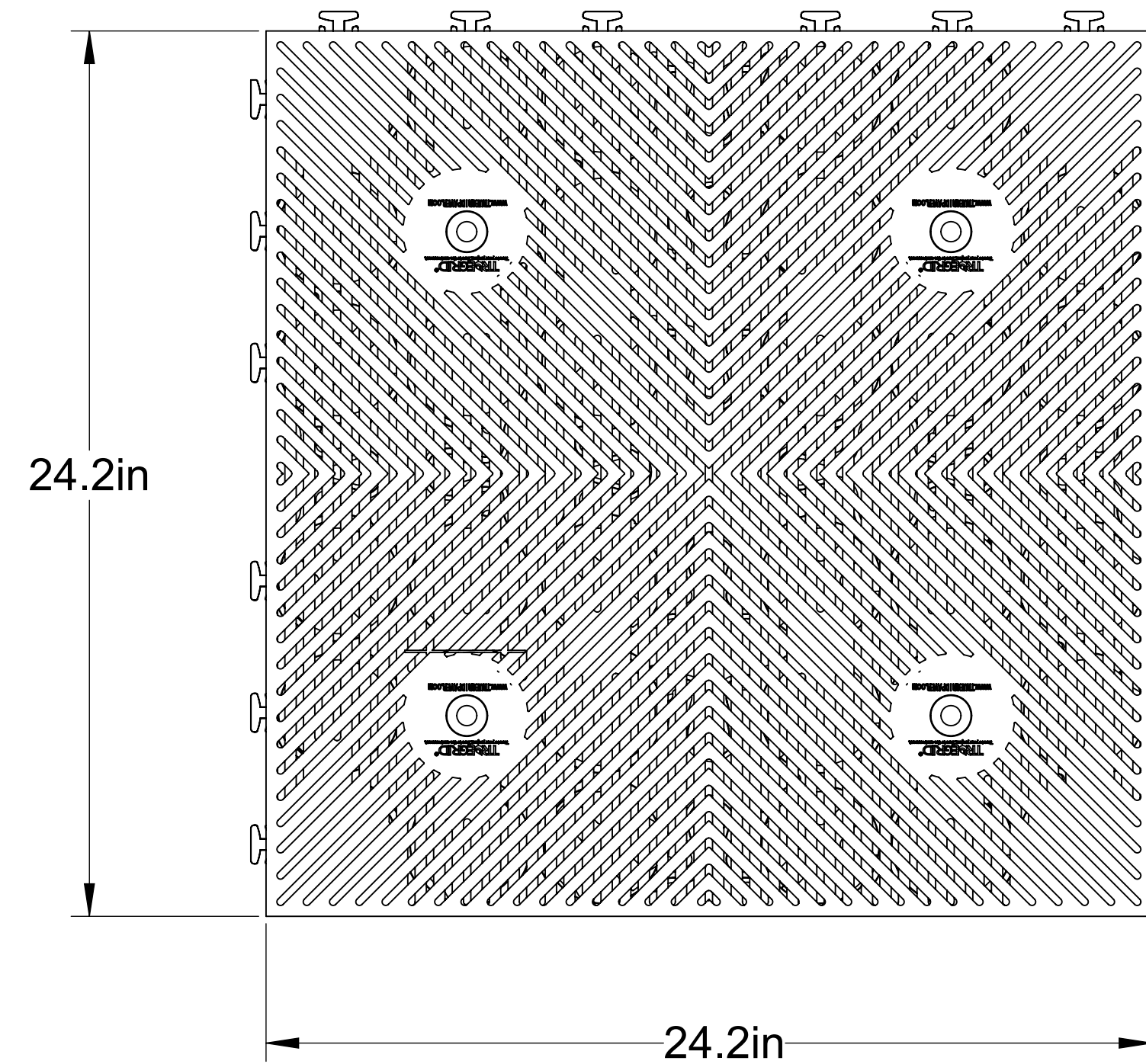
TOP VIEW
